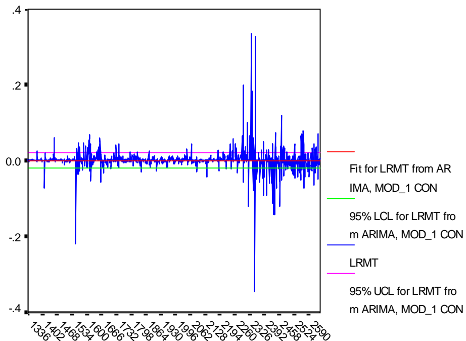
FIGURE 1.1. BUILDING UP PREDICTIVE MODEL (ARIMA, 2,0,1) FOR THE HISTORICAL PERIOD (1-1335) AND FORECASTING THE VALIDATION PERIOD (1336-2638).
